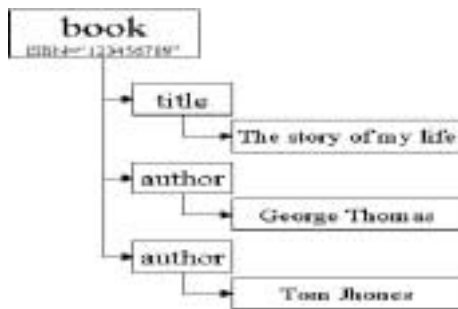
Figure 1. Sample DOM tree.
